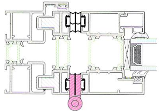
Outer Frame Detail with Adjustable Jamb
